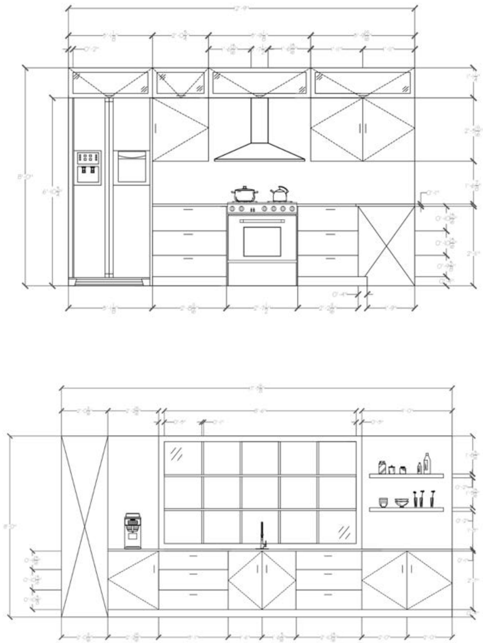
kitchen elevations
