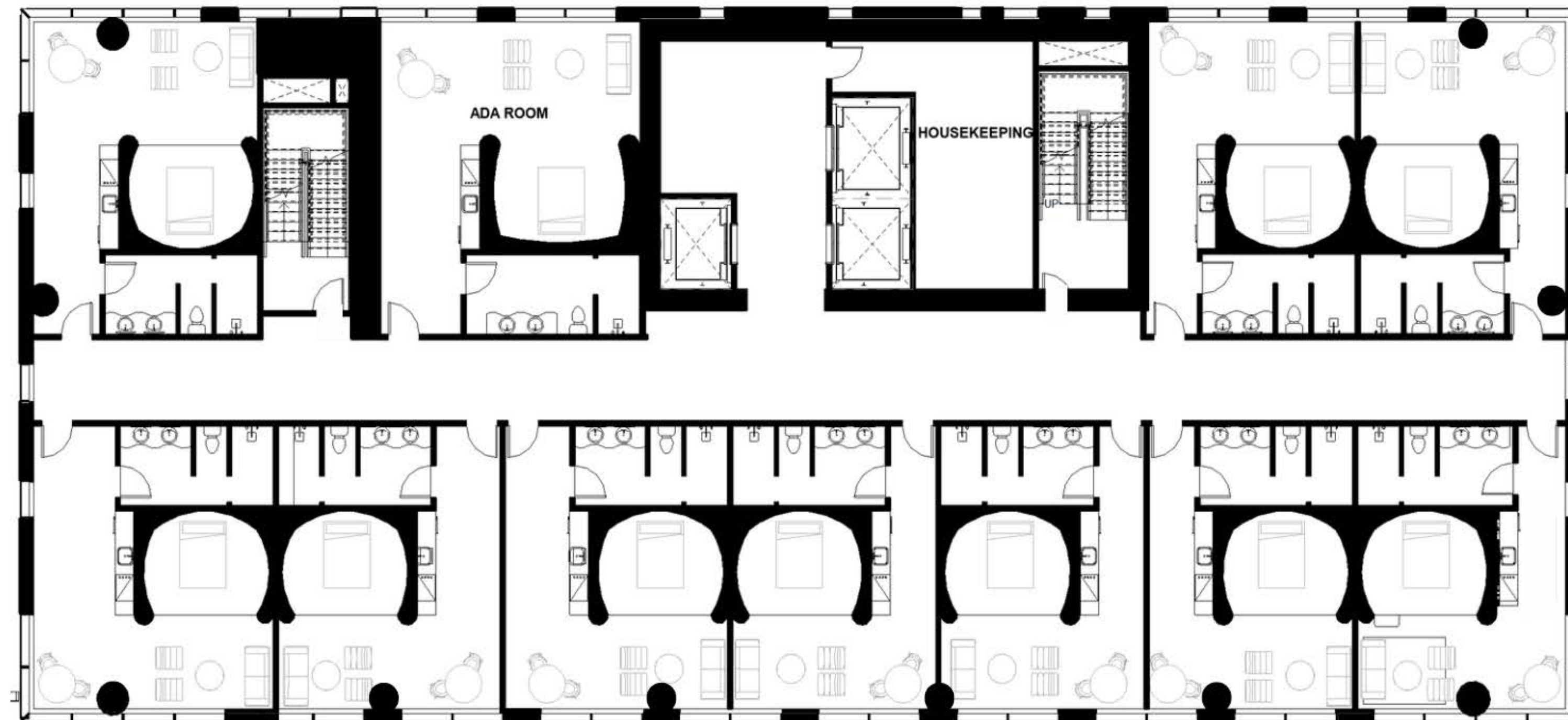
typical floorplan
